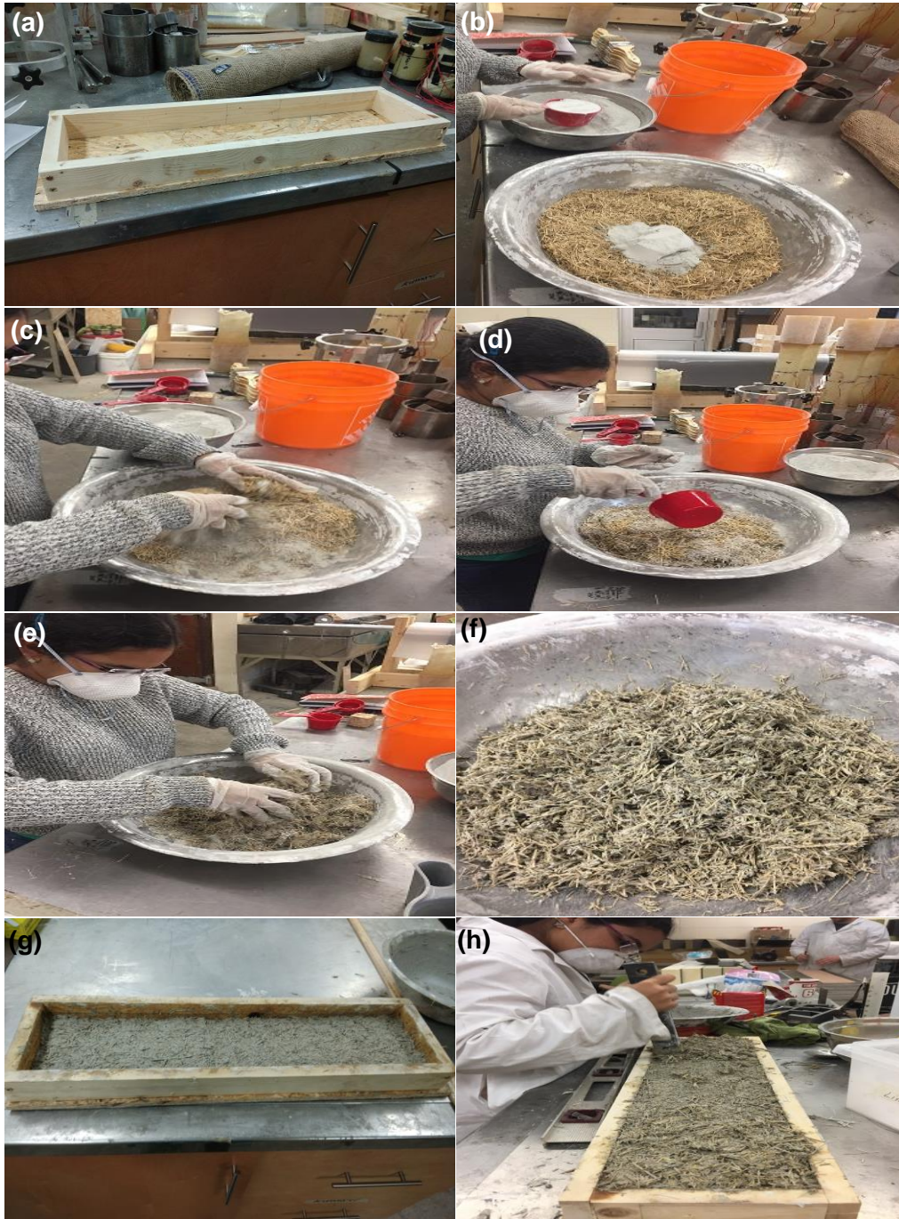
Figure 1: Specimen preparation: (a) formwork; (b) adding binder to flax; (c) mixing binder with flax; (d) adding water to mix; (e) mixing water with flax and binder; (f) finally obtained mix; (g) formwork filled to half to place burlap; and (h) casting and compaction
