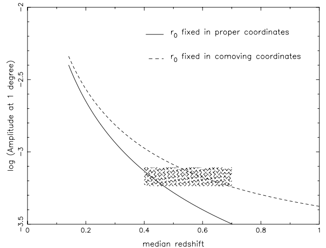
FIG. 3.—Change of the angular correlation amplitude with the sample median redshift based on Limber integration. Here we use a form of selection function (Baugh et al. 1996) that has been studied in K -band surveys and assumed a spatial correlation amplitude estimated from a 3.6 \mu\text{m} SWIRE sample. The two evolution models for galaxy clustering along with the uncertainties from our angular correlation amplitude measurement place a constraint on the median redshift of the 3.6 \mu\text{m} sample in the FLS survey.
