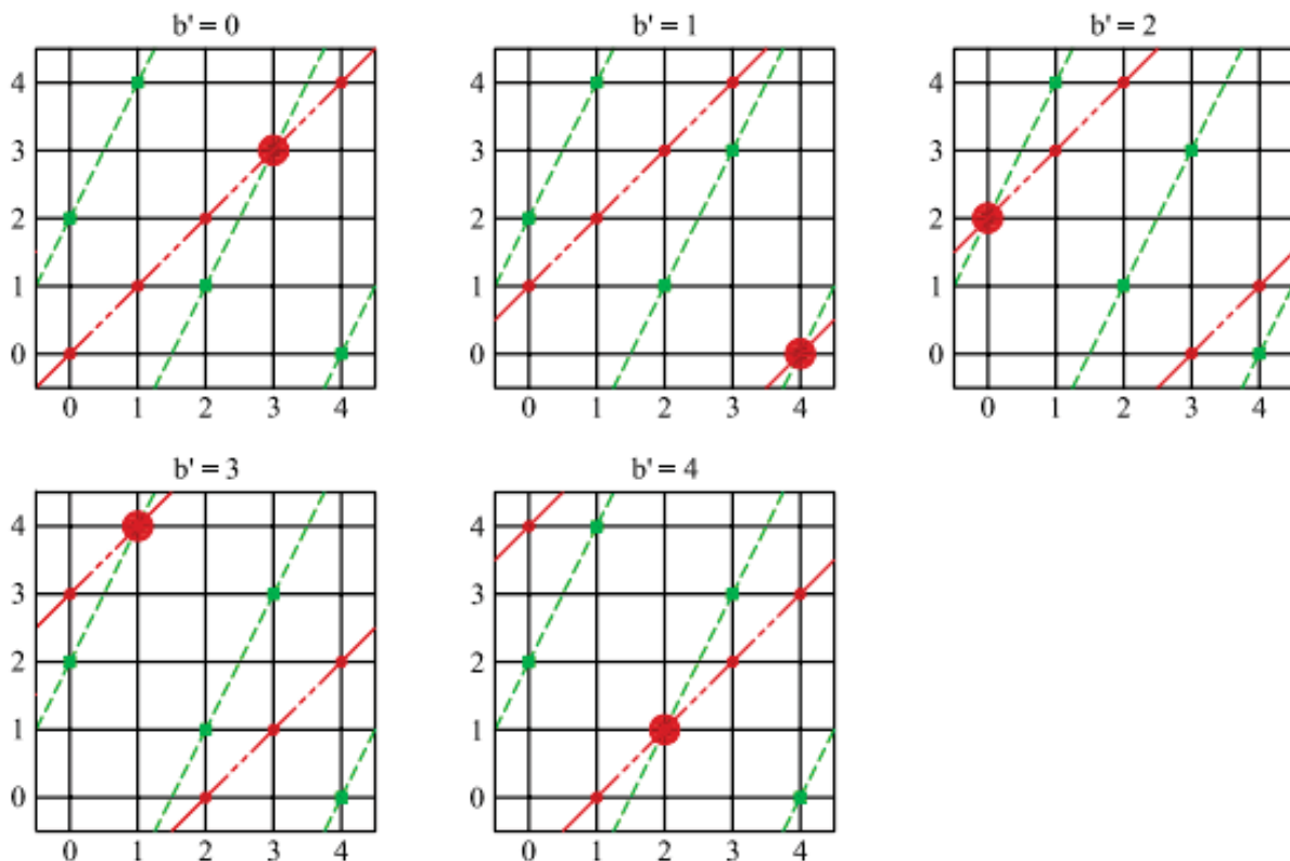
Figure 3.2: Given a signed message ( m = 2, b = 2 ) and a desired fake message ( m' = 1 ), each possible forged offset ( b' ) matches only one of the possible verifiers. Since the verifier is chosen at random, the chance of successful forging is \frac{1}{|\mathbb{F}|} .
